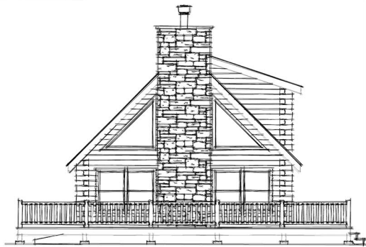
LEFT ELEVATION
