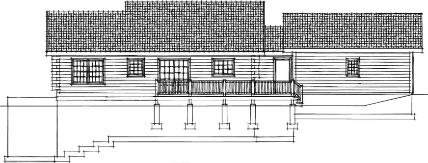
REAR ELEVATION
