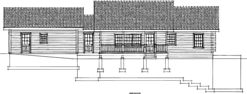
FRONT ELEVATION
