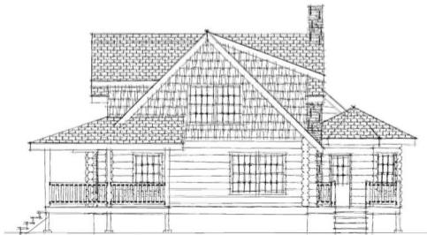
LEFT ELEVATION
