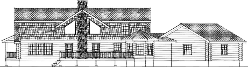
REAR ELEVATION
